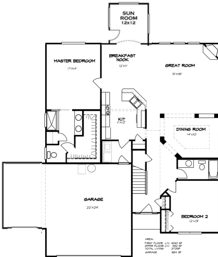
FIRST FLOOR ELECTRICAL PLAN
